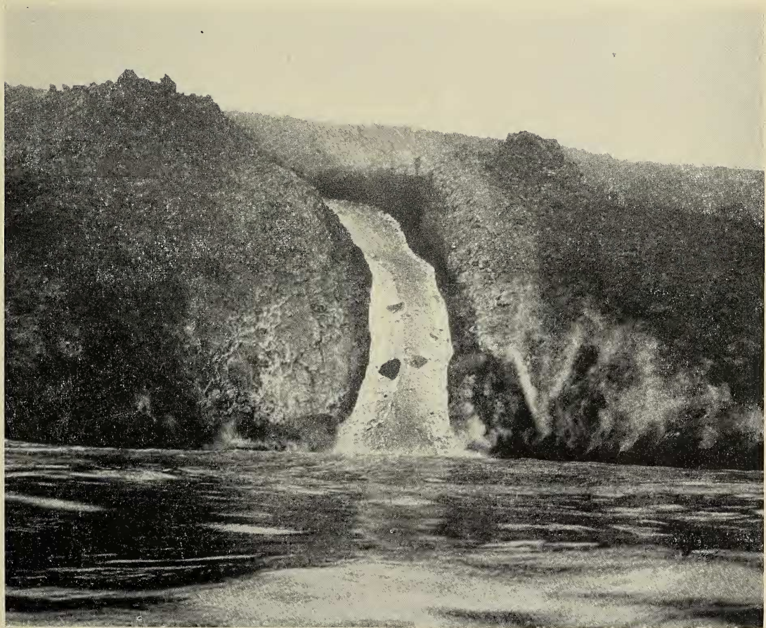
FIG. 3. The third lava flow entering the water several days later. Photograph by Jack Matsumoto.
